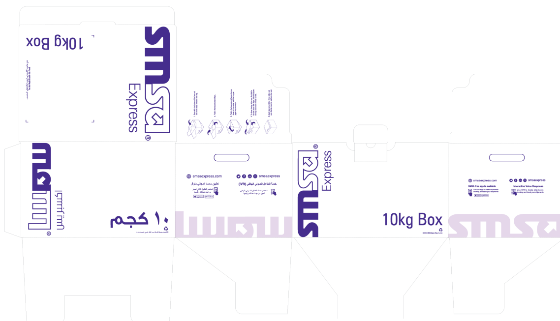
SMSA Box - 10Kg (P.P New Dimension - 40.5 x 33.5 x 25.5cm, Pre Print 2 Colors, DW-EB-Glued
